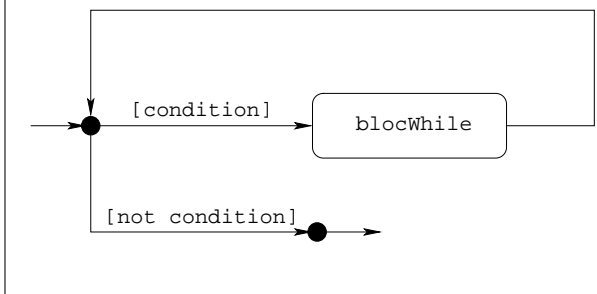
Fig. 2.15 : BOUCLE while while condition : blocWhile
